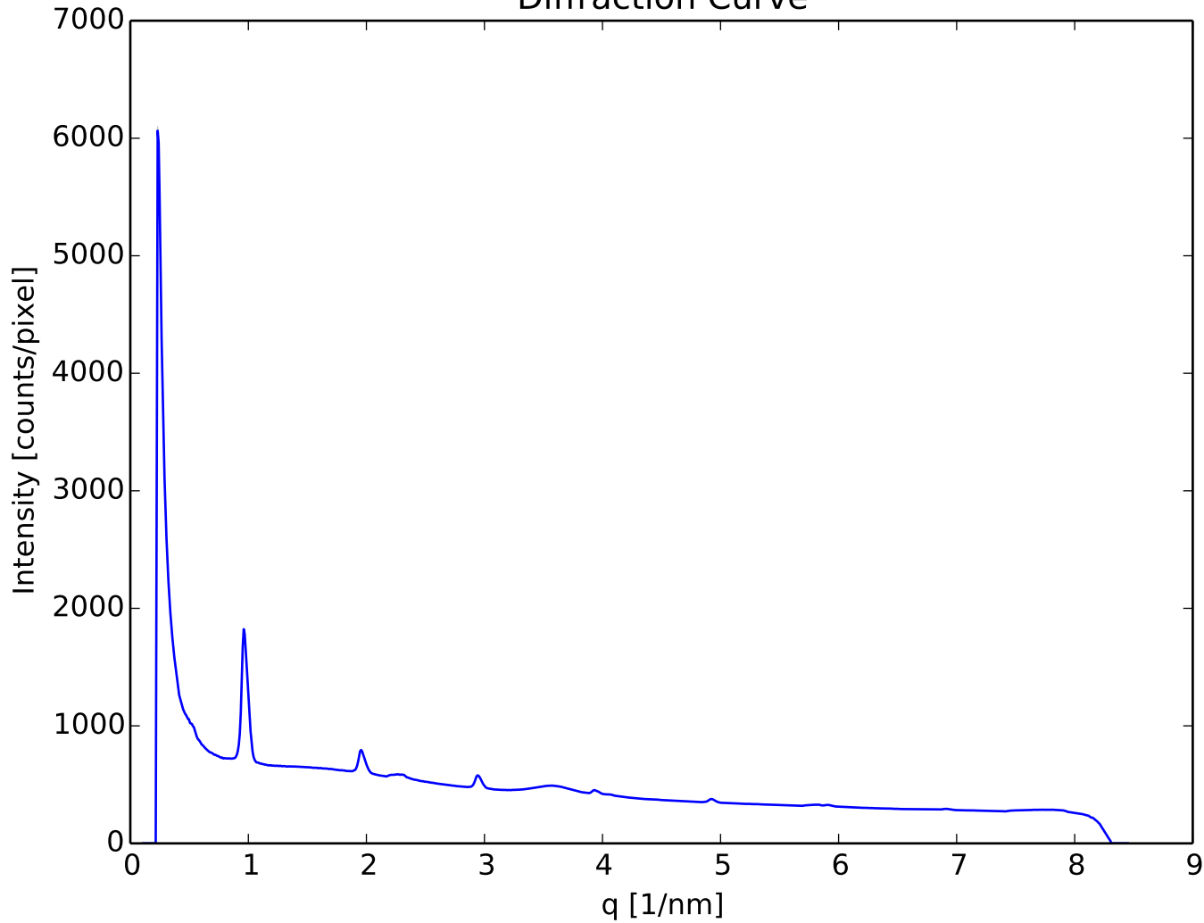
Diffraction Curve
